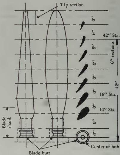
FIGURE 7-2. Typical propeller blade elements.
